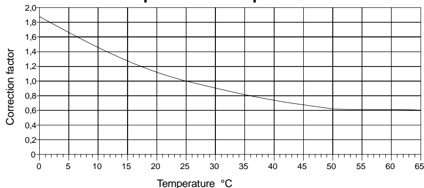
Temperature compensation
